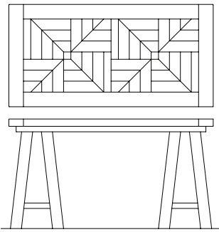
468-415 Writing Desk 56W x 28D x 30H in. Shown on pages 8, 9
