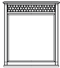
472-05M Fretwork Landscape Mirror 39.5W x 2.25D x 42.75H in. Shown on pages 6, 7
